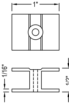
DETAIL ALUMINUM HIDDEN H-CLIP 599 MAGNI-COATED
