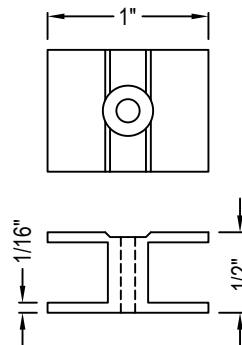
DETAIL ALUMINUM HIDDEN H-CLIP 599 MAGNI-COATED
