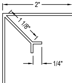
DETAIL A ALUMINUM EXTRUSIONS INSIDE CORNER (ANODIZED, PAINTABLE)
