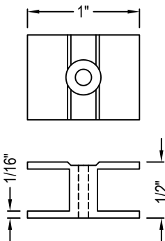
DETAIL ALUMINUM HIDDEN H-CLIP 599 MAGNI-COATED
