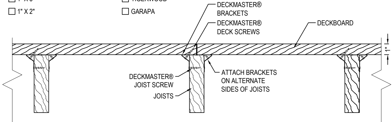
SECTION UNDER MOUNT DECK FASTENER
