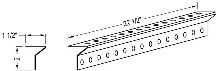
SECTION UNDER MOUNT DECK FASTENER
